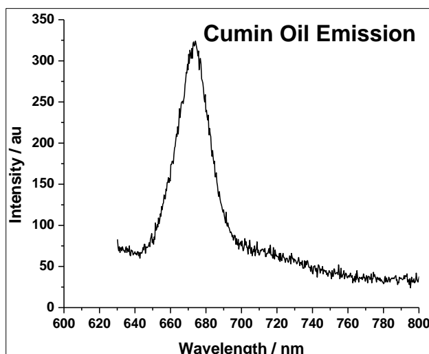
Fig 2: N. Sativa Oil Emission excited by He-Ne Laser (632.8 nm)
