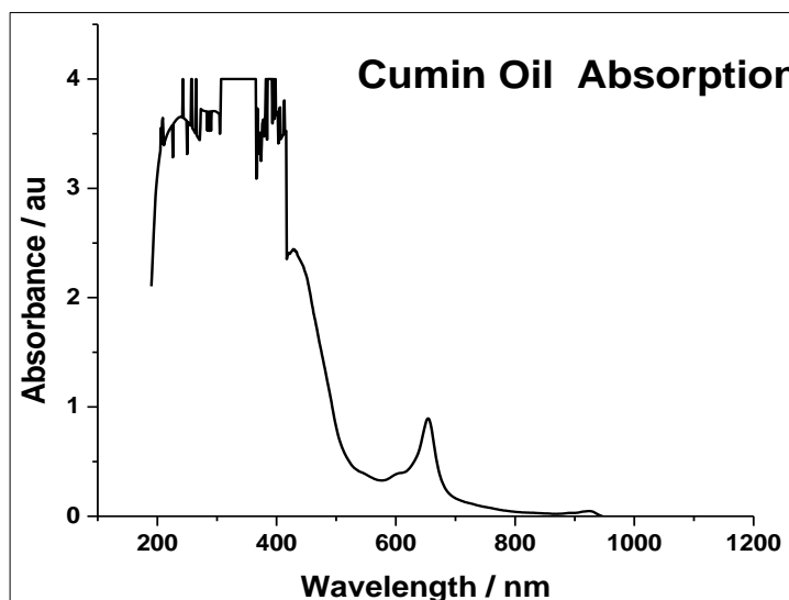
Fig 1: N. Sativa Oil Absorption
