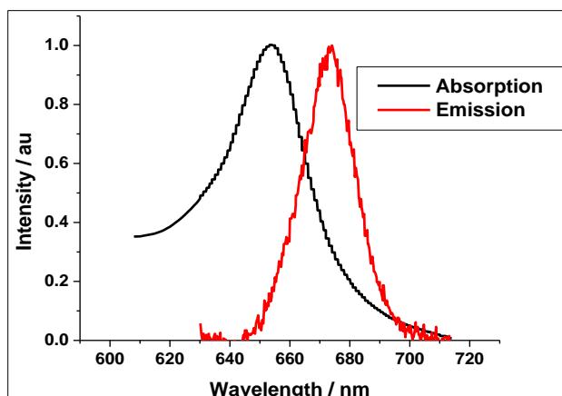
Fig 3: N. Sativa Oil Absorption and Emission
