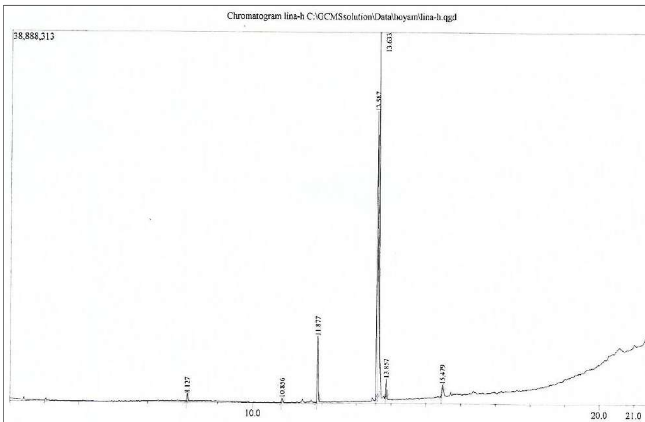
Fig 4: GC/MS analysis compounds of N. Sativa oil
